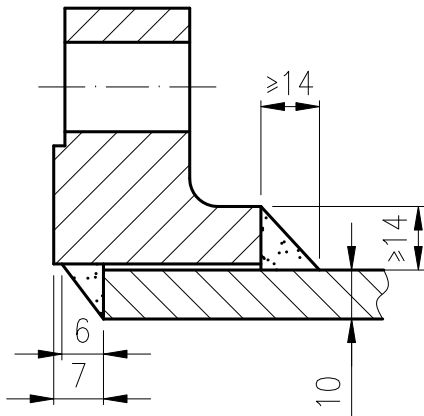
Welding detail for flange to pipe 法兰与接管焊接视图
