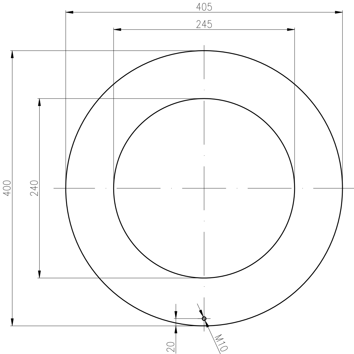
Developed pattern 展开图
